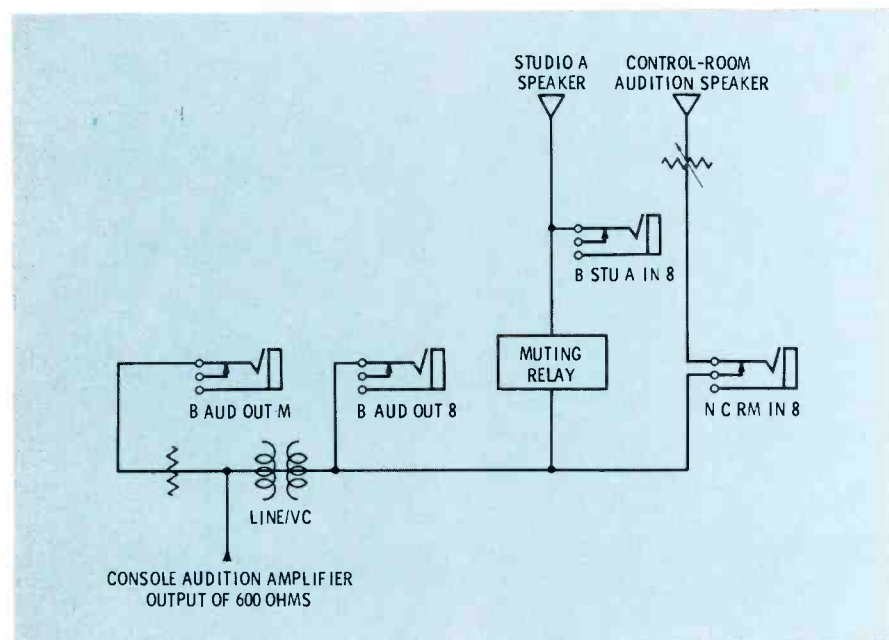
Fig. 5. Simplified circuit of console audition amplifier jacks in patch panel.
