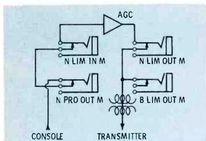
Fig. 4. Several connections to AGC amplifier are possible through jacks.
